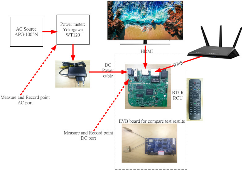
Block Diagram
